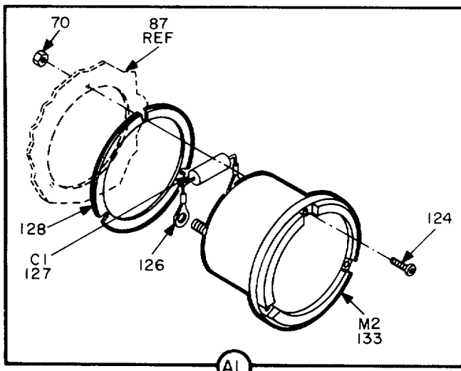
Figure 1. Amplifier-Mixer 6704/TSC (Sheet 9 of 9).
